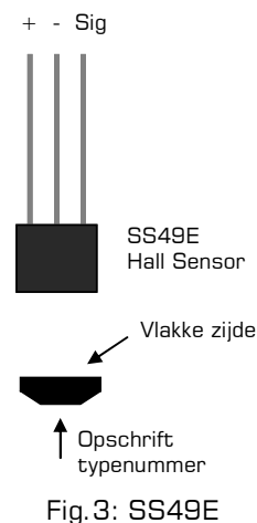
Fig.3: SS49E
